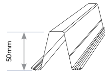
50 mm TOP HAT – 0.95 BMT: 50TH0.95 (1.37kg/m)
