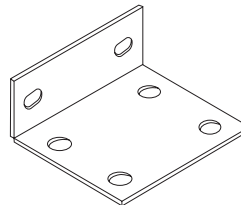
General Purpose Bracket - C200: GPB200 (0.23kg/ea)
