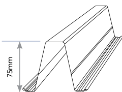
75 mm TOP HAT – 0.75 BMT: 75TH0.75 (1.41kg/m)
