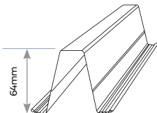
64 mm TOP HAT – 0.95 BMT: 64TH0.95 (1.58kg/m)
