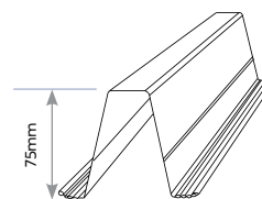
75 mm TOP HAT – 0.95 BMT: 75TH0.95 (1.77kg/m)
