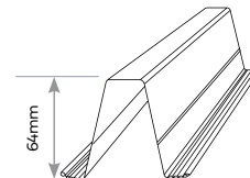
64 mm TOP HAT – 1.15 BMT: 64TH1.15 (1.91kg/m)
