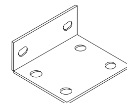
General Purpose Bracket - C300: GPB300 (0.23kg/ea)
