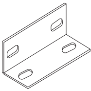
Angle Connector - C150: MF-AC150 (0.30kg/ea)
