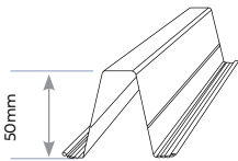
50 mm TOP HAT – 1.15 BMT: 50TH1.15 (1.63kg/m)
